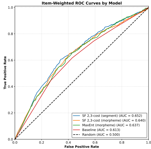
Figure 4: Item-weighted AUC-ROC curves by model.
